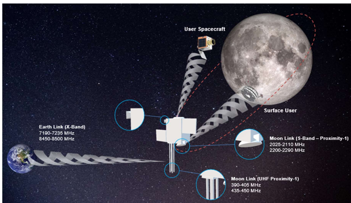
Figure 11: Lunar Pathfinder Earth and Moon links
