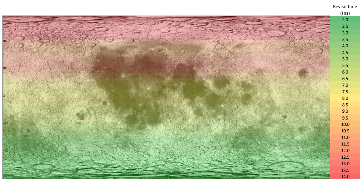
Figure 10: Average revisit time over 1 year.
