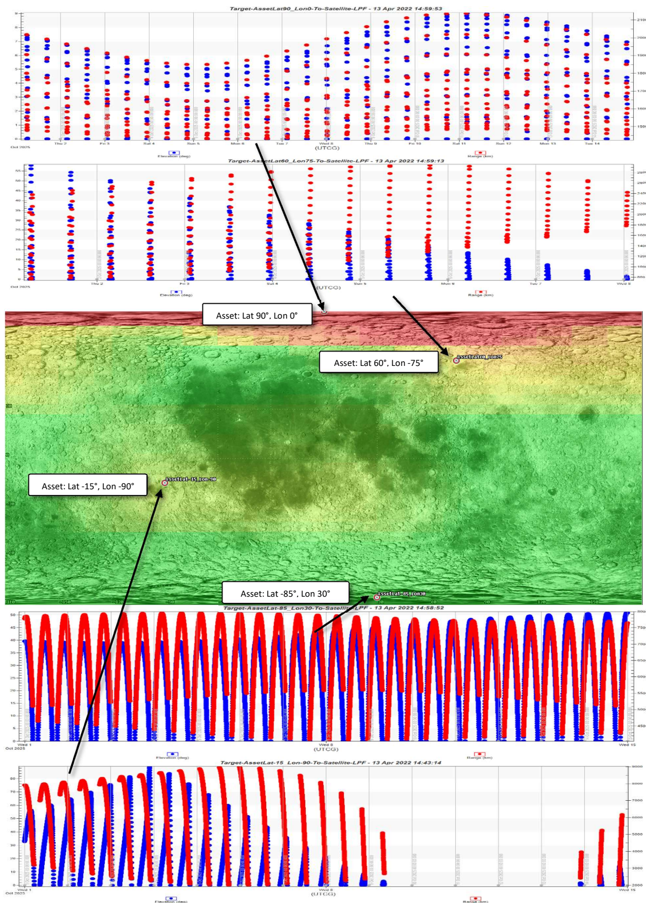
Figure 7: Maximum revisit time over a 14 day Earth period. Elevation and range of Lunar Pathfinder from 4 locations have also been plotted to further explain the nature of the coverage gaps.
