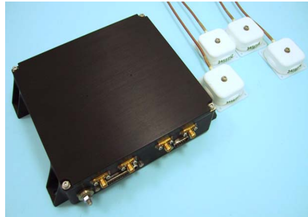
SGR-20 GPS Receiver and Antennas
